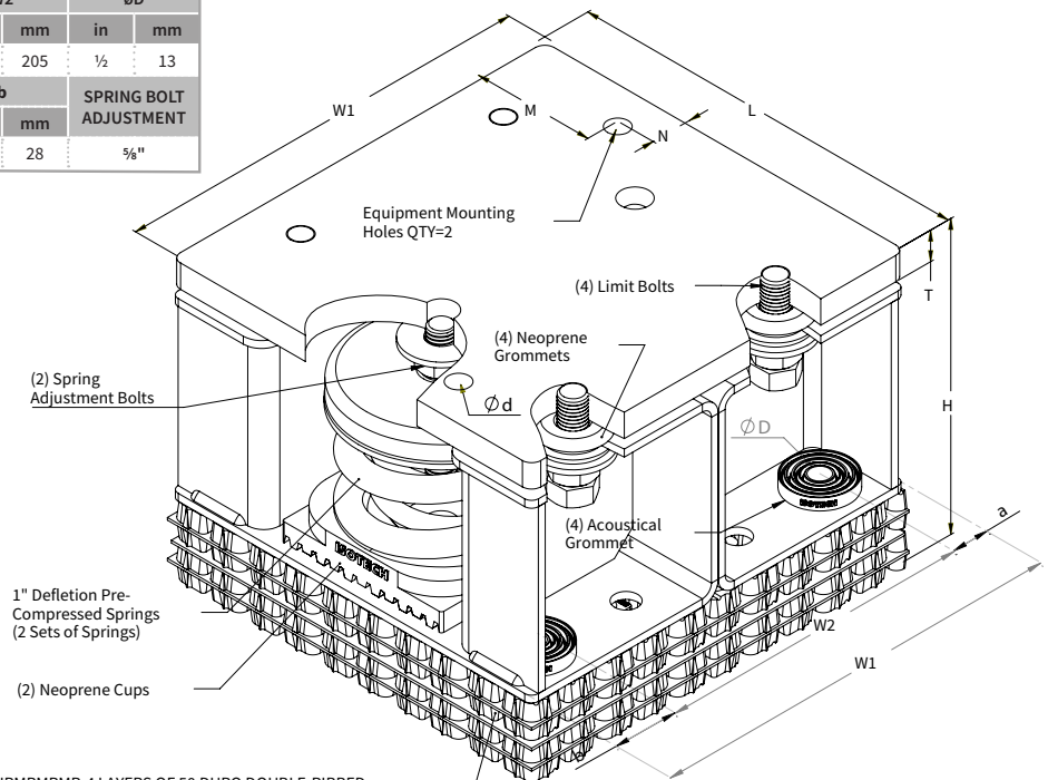
IRMRMR-4 LAYERS OF 50 DURO DOUBLE-RIBBED NEOPRENE PADS- SEPARATED WITH GALVANIZED STEEL
