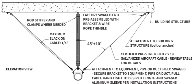
ATTACHMENT BRACKET TYPE: ANCH. BRACKET
